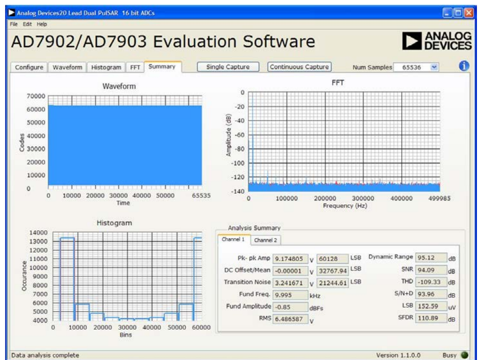
Figure 25. Summary Tab
