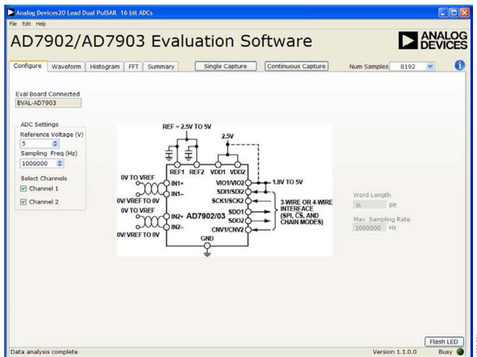
Figure 21. Main Window
