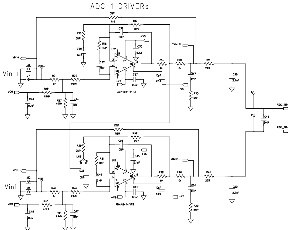
Figure 26. Schematic, Page 1
