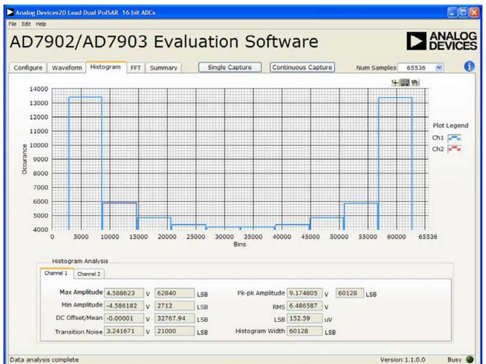
Figure 23. Histogram Tab
