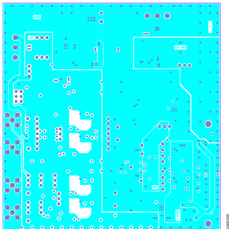
Figure 35. EVAL-AD7903SDZ Evaluation Board Layer 3—Power
