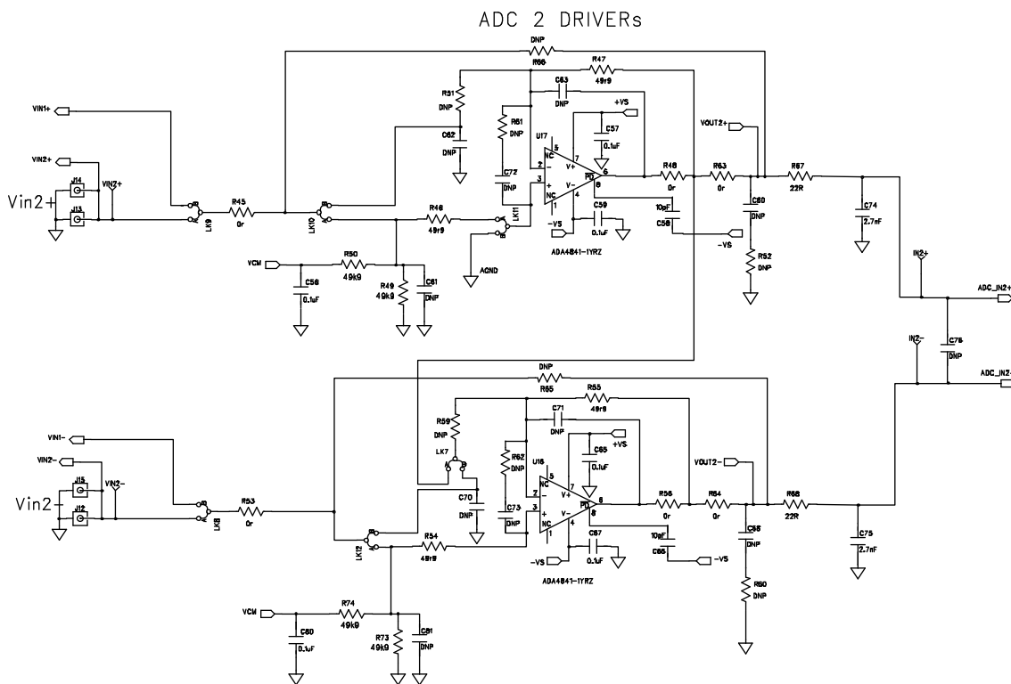
Figure 27. Schematic, Page 2
