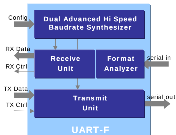
Figure 2: UART-F Structure
