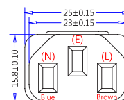
ME-302 (IEC 60320, C13, 10A 250V~) (Dimensions of Connector Face)
