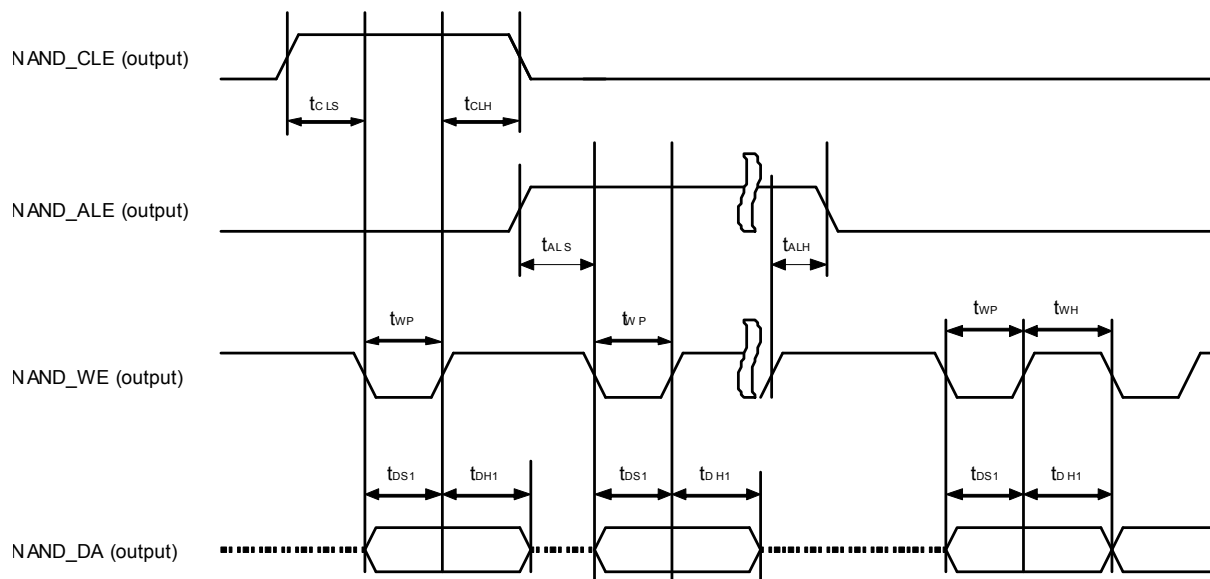
Figure 2-21. NAND Flash Interface Timing 1
