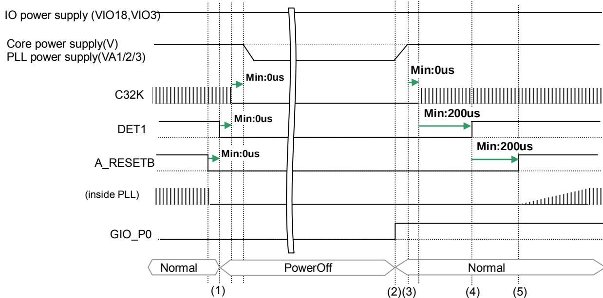
Figure 2-7. PowerOff Normal timing
