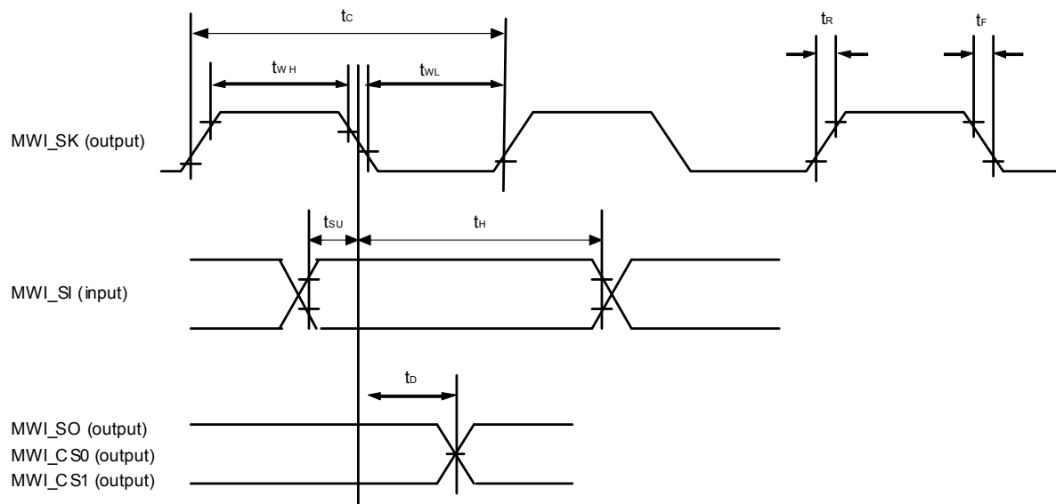
Figure 2-24. MICROWIRE Interface Timing
