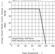
Figure 2- Forward Derating Curve
