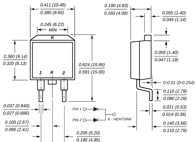
TO-263AB (MBRB30H90CT, MBRB30H100CT)
