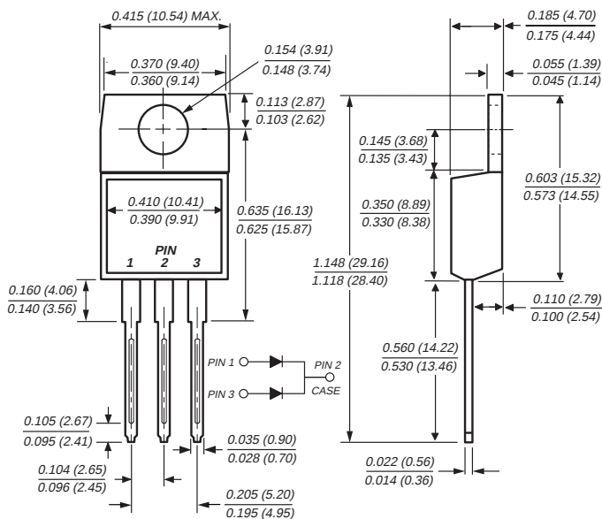
TO-220AB (MBR30H90CT, MBR30H100CT)
