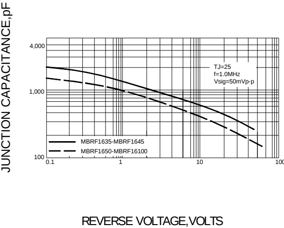
FIG.5-TYPICAL JUNCTION CAPACITANCE
