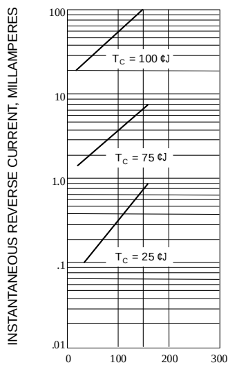
Fig. 3-TYPICAL REVERSE CHARACTERISTICS
