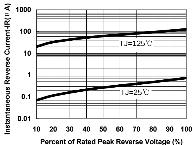
Fig.2-Typical Reverse Characteristics
