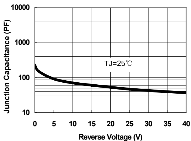
Fig.1-Typical Junction Capacitance
