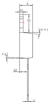
TO-220AB
