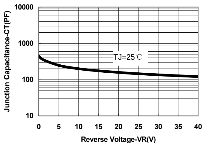
Fig.1-Typical Junction Capacitance
