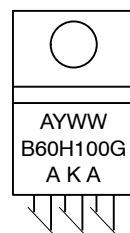
TO-220AB CASE 221A PLASTIC
