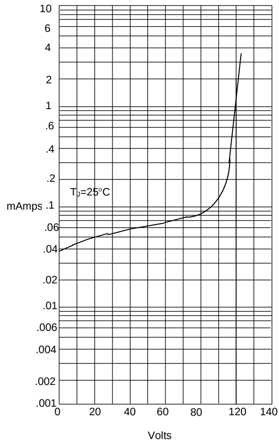
Figure 1 Typical Reverse Characteristics
