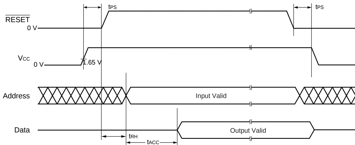
Power ON/OFF Timing Diagram
