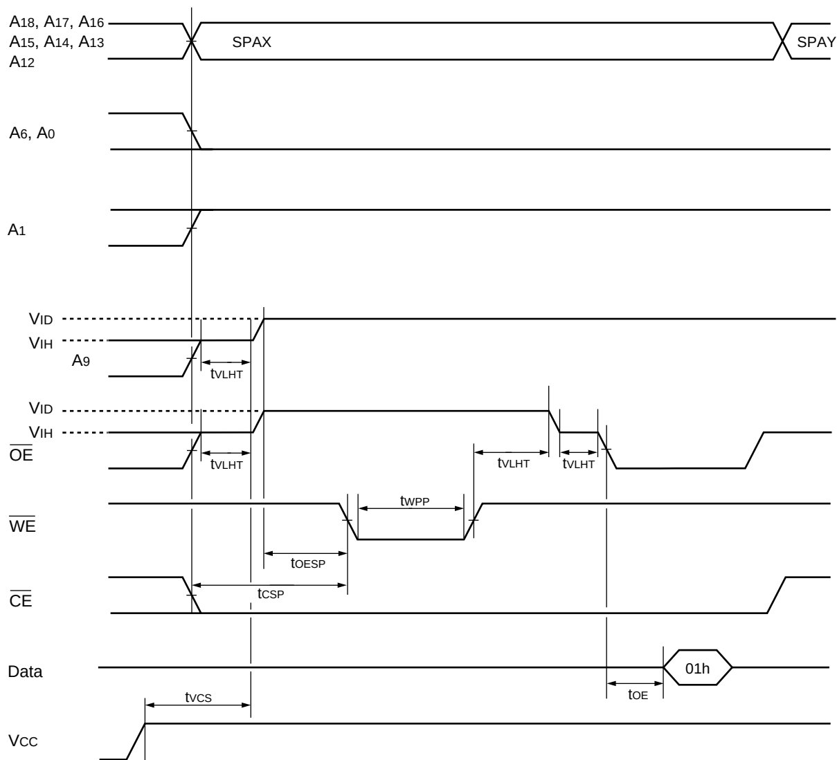
(13) Sector Protection Timing Diagram
