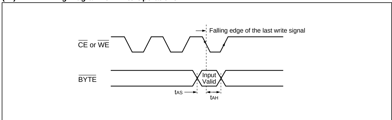
(12) \overline{\text{BYTE}} Timing Diagram for Write Operations
