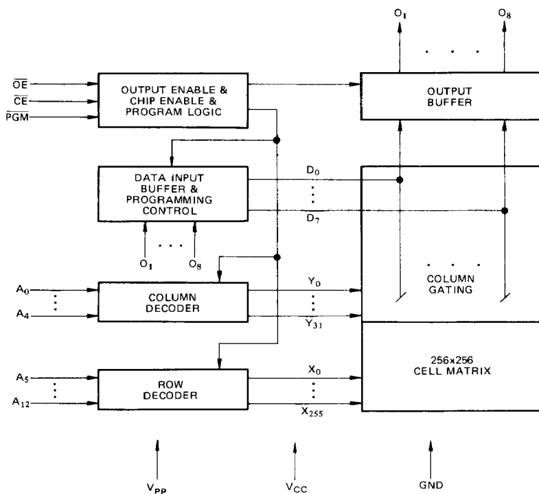
Fig. 1 — MBM 2764 BLOCK DIAGRAM
