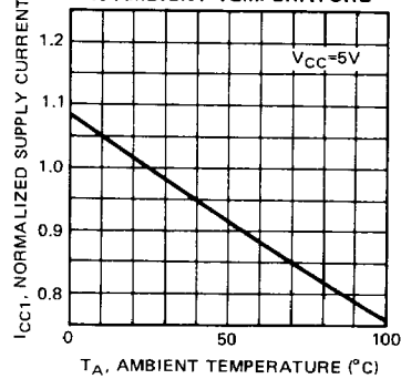
Fig. 4 — SUPPLY CURRENT (STANDBY) vs AMBIENT TEMPERATURE
