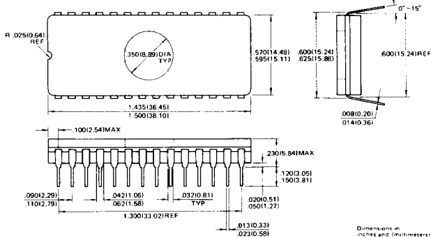
28-LEAD CERAMIC (CERDIP WITH TRANSPARENT LID) DUAL IN-LINE PACKAGE (CASE No.: DIP-28C-C01)
