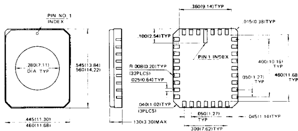
32-PAD CERAMIC (METAL SEAL) LEADLESS CHIP CARRIER (CASE No.: LCC-32C-A01)
