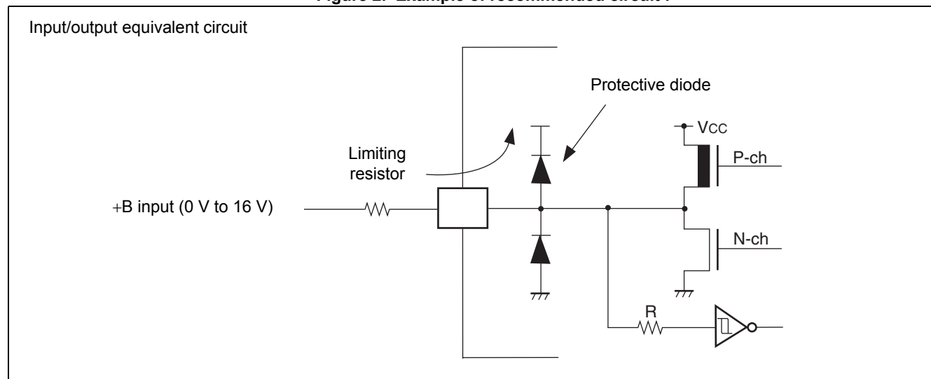
Figure 2. Example of recommended circuit :
