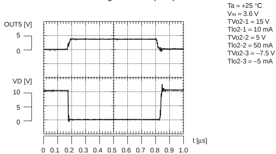
Switching waveform (CH5)
