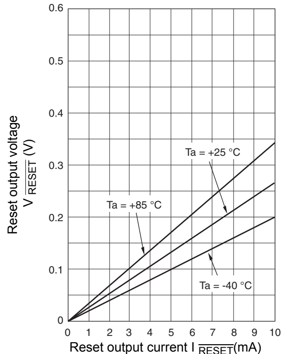
V_{\overline{RESET}} - I_{\overline{RESET}} characteristics (N-MOS side)
