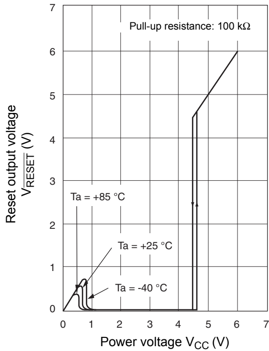
\overline{V_{RESET}} - V_{CC} characteristics
