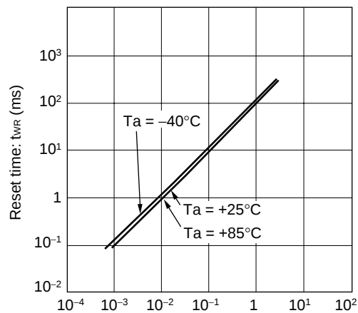
Reset time- C_{TP} capacitance
