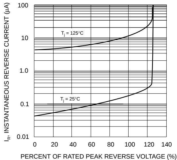
Fig. 5 Typical Reverse Current
