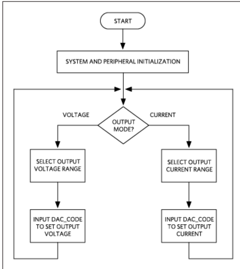
Figure 2. The Carmel firmware flowchart.
