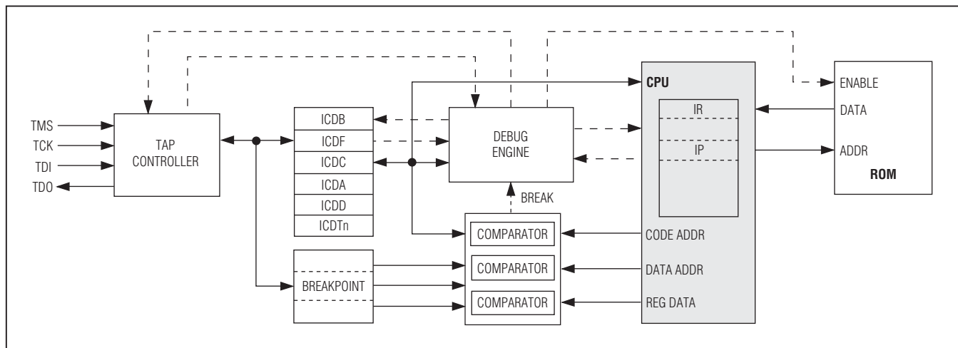
Figure 12-1. In-Circuit Debugger
