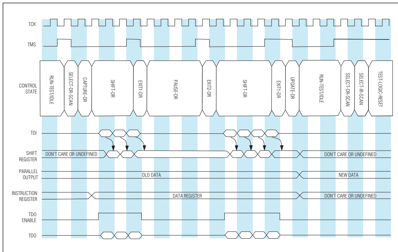
Figure 11-4. TAP Controller Debug Mode DR-Scan Example
