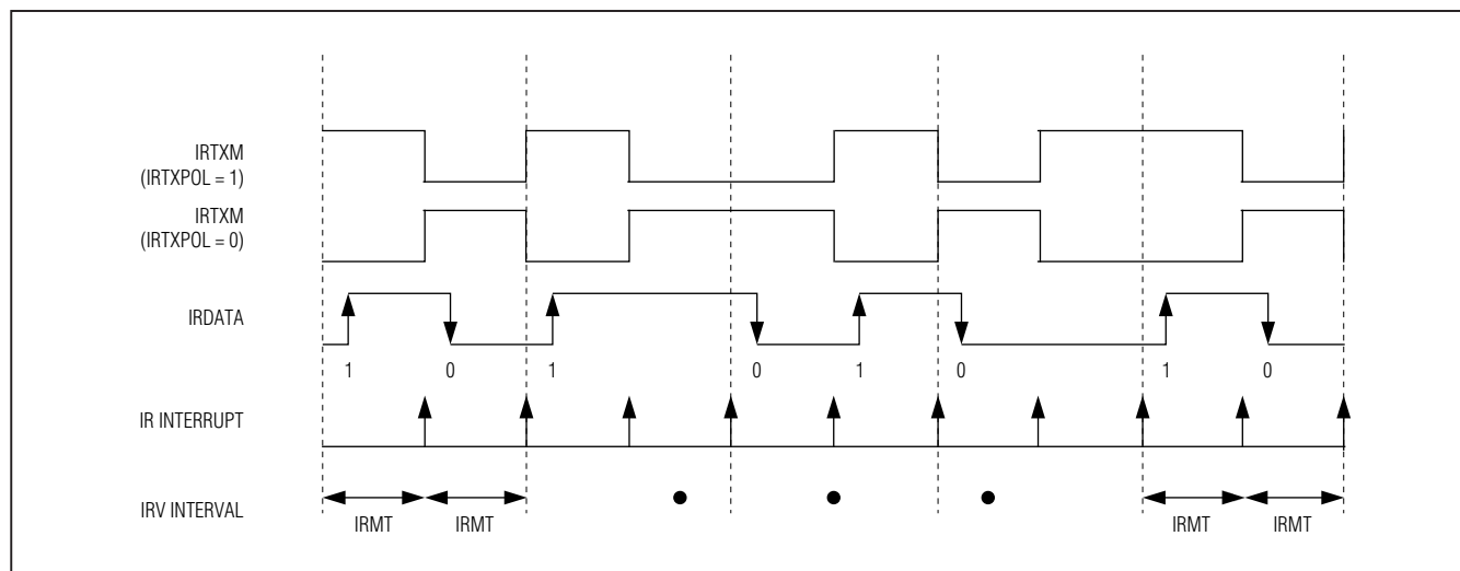
Figure 8-4. External IRTXM (Modulator) Output
