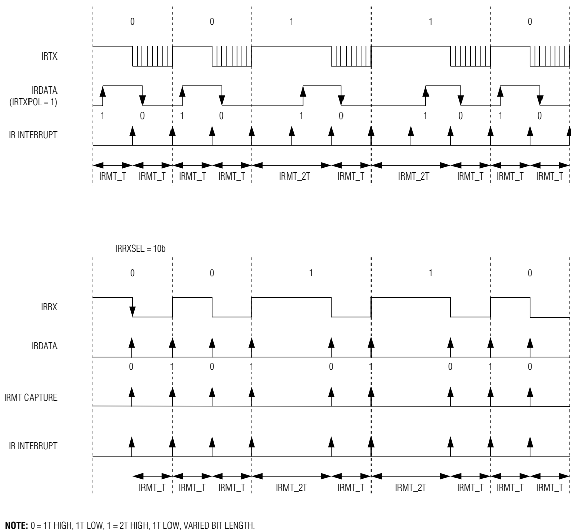
Figure 8-8. Sony Remote Encoding Example
