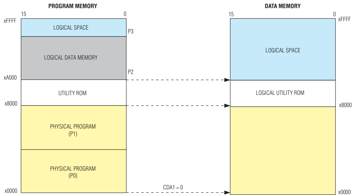
Figure 2-4. CDA Functions in Word Mode
