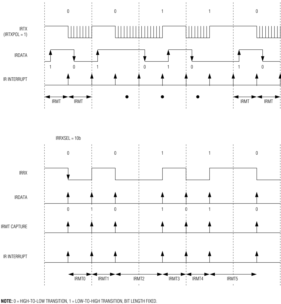
Figure 8-7. Philips Remote Encoding Example
