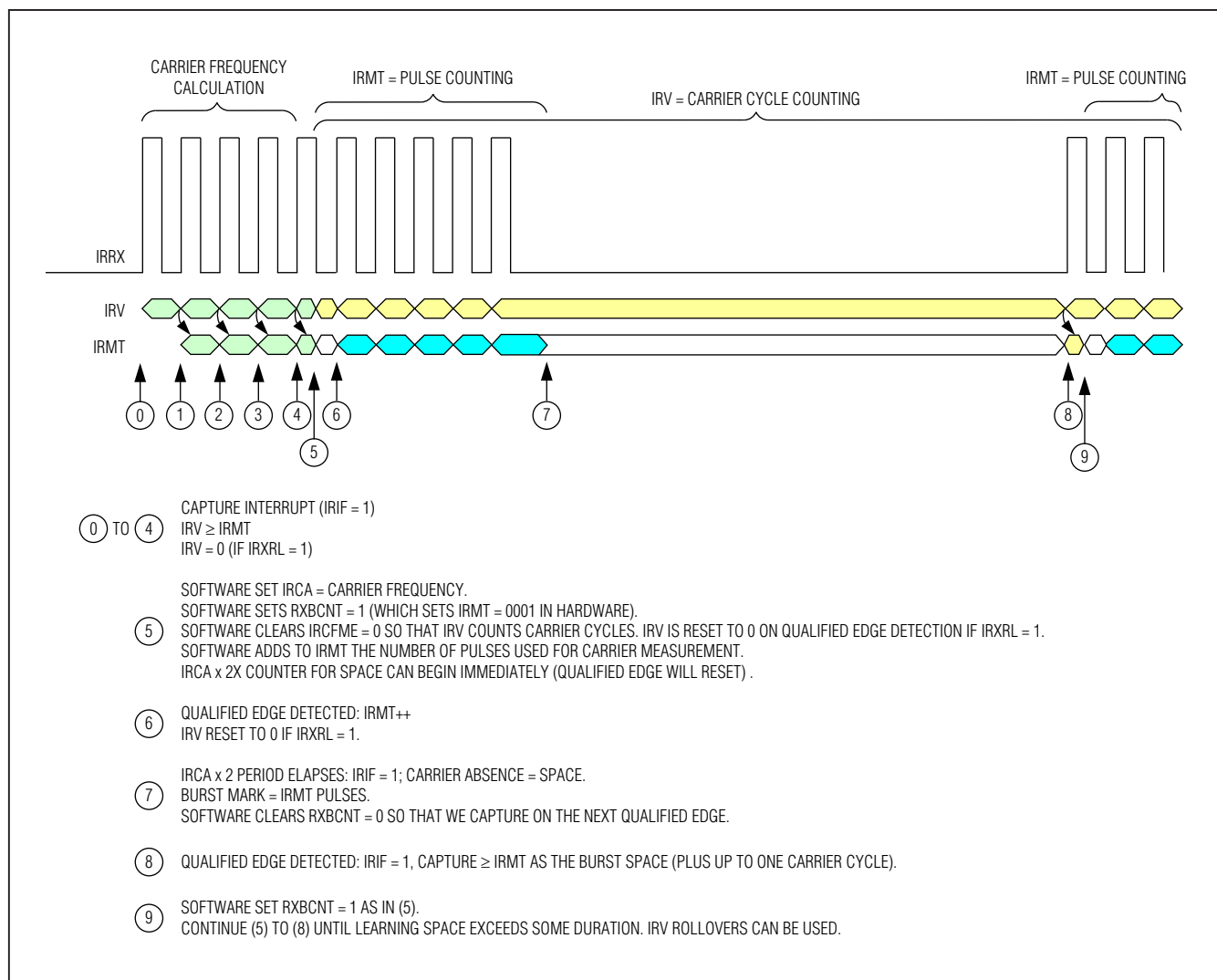
Figure 8-6. Receive Burst-Count Example
