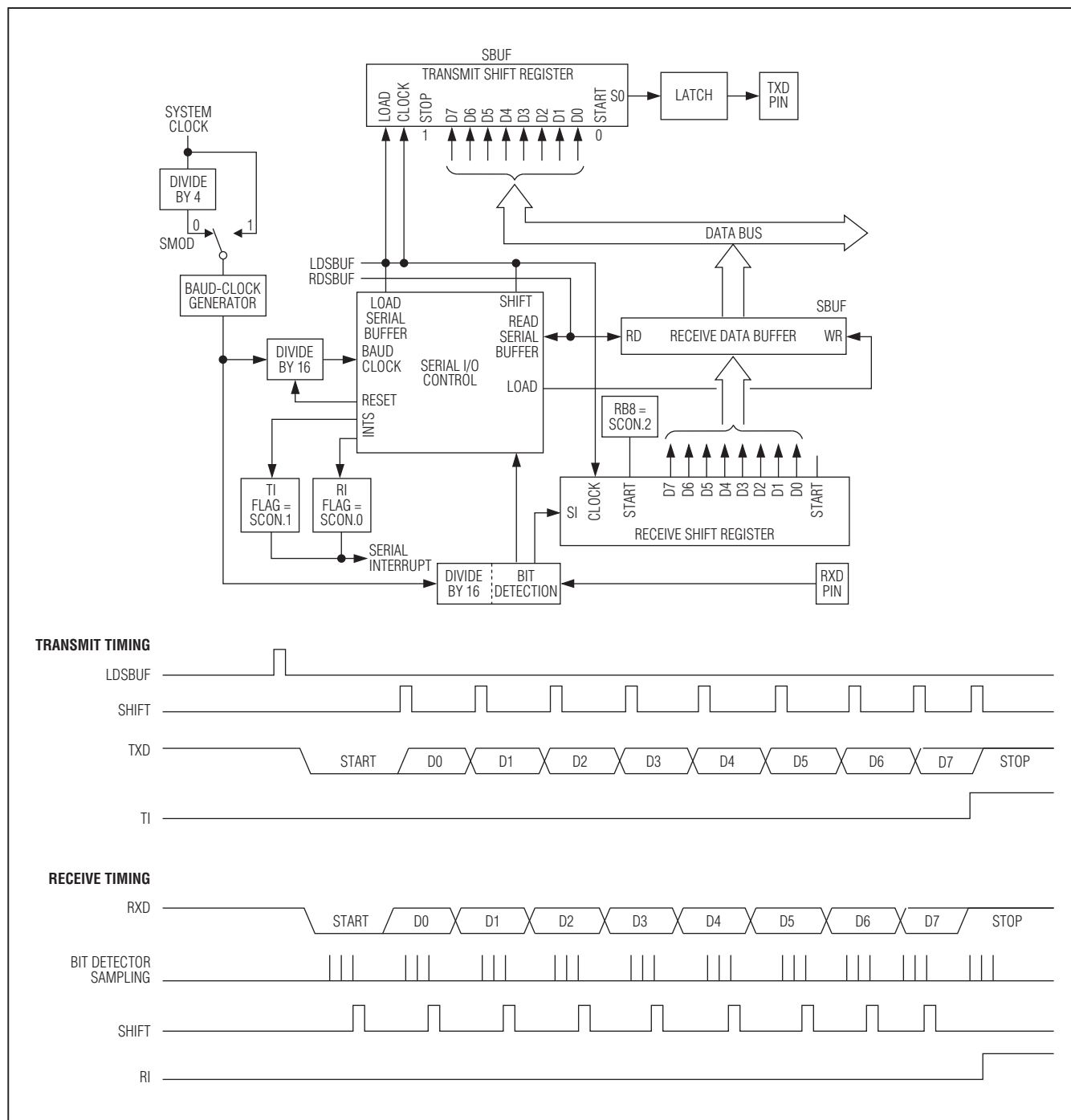
Figure 9-2. USART Mode 1
