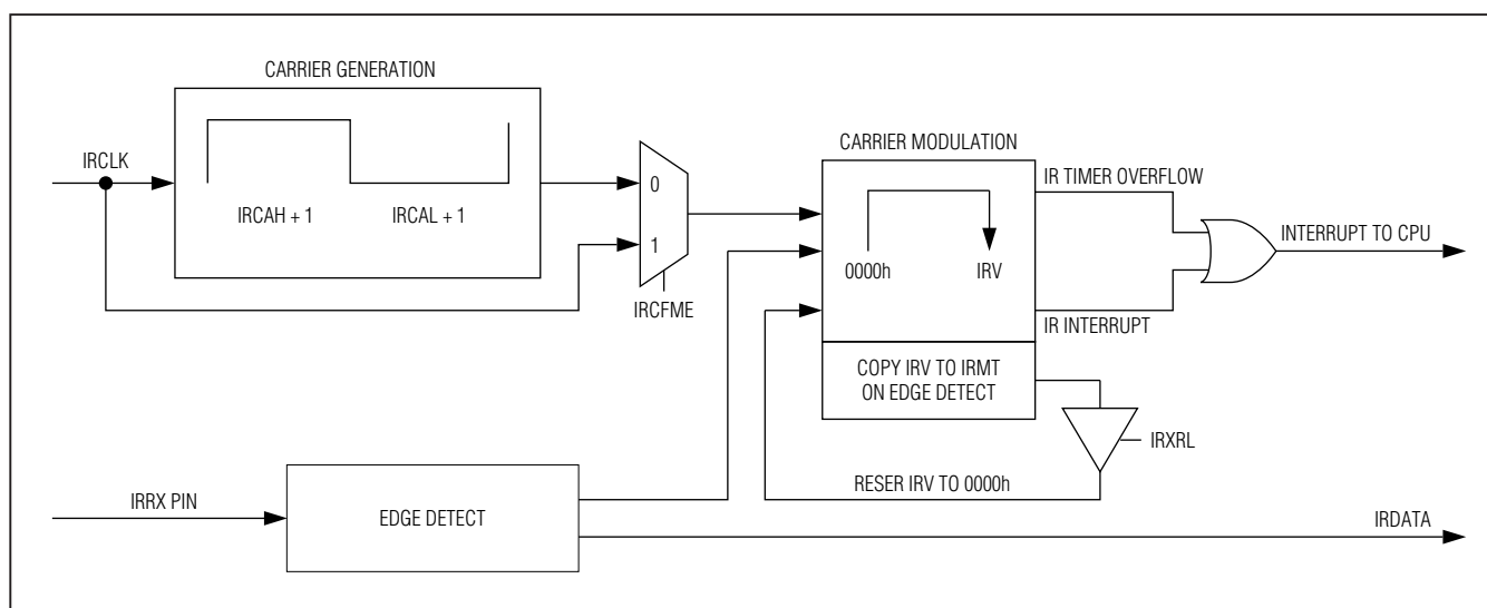
Figure 8-5. IR Capture
