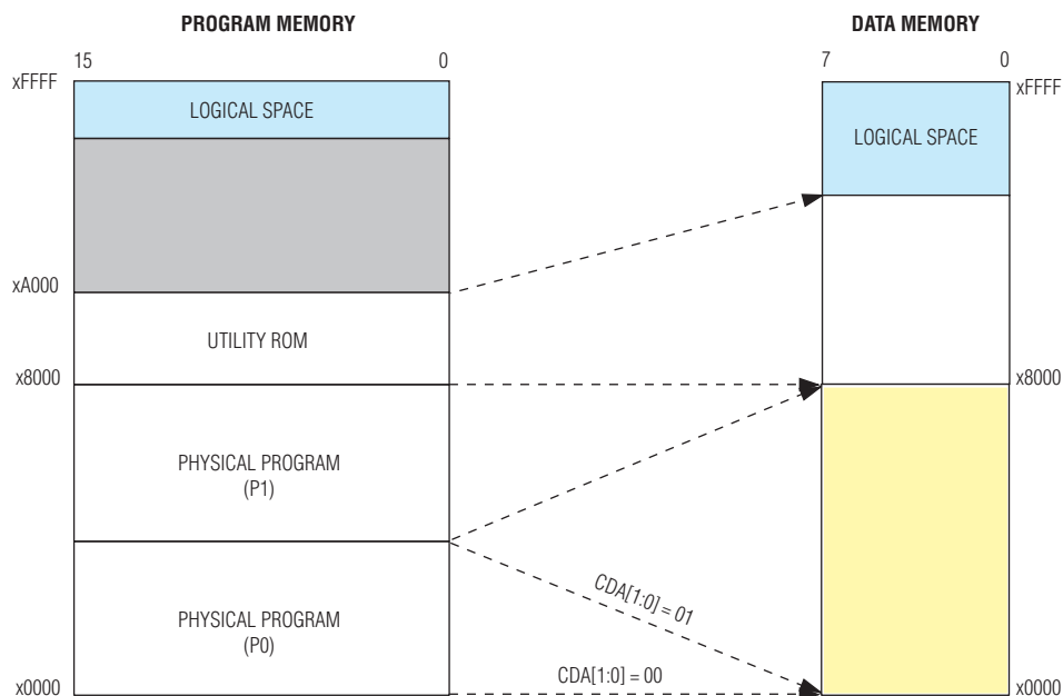
Figure 2-5. CDA Functions in Byte Mode
