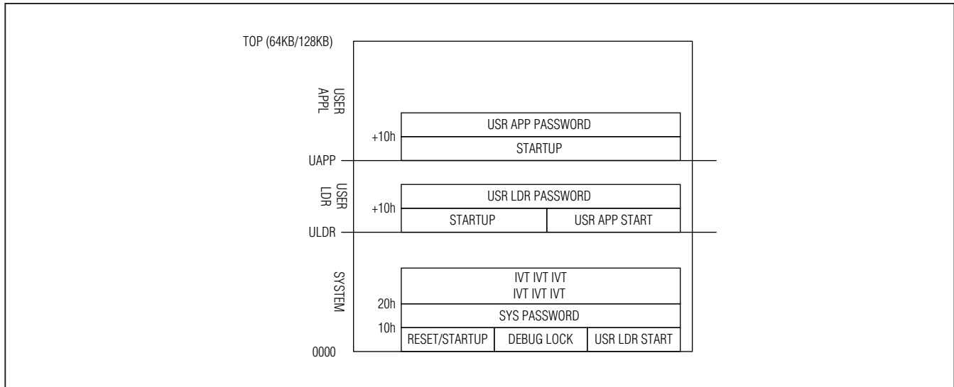
Figure 2-7. Overview of Memory Regions
