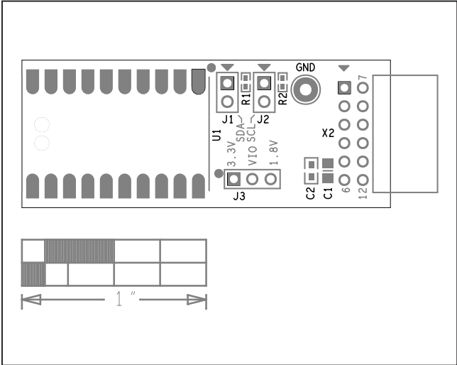
MAXPICO2PMB Adapter Board PCB Layout—Top Silkscreen
