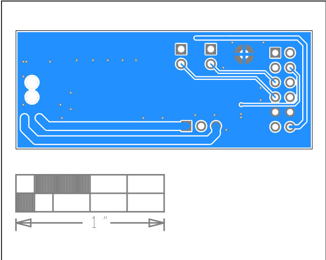
MAXPICO2PMB Adapter Board PCB Layout—Bottom
