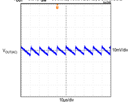
MAXM17630/MAXM17632 STEADY-STATE OUTPUT-VOLTAGE RIPPLE V_{OUT} = 3.3V , f_{SW} = 900kHz , 10mA LOAD, DCM MODE
