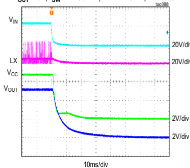
MAXM17631/MAXM17632 SHUTDOWN THROUGH V_{IN} V_{OUT} = 5V , f_{SW} = 1250kHz , 10mA LOAD, PFM MODE
