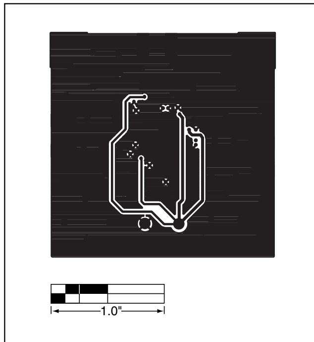
Figure 7. MAX9989/MAX9990 EV Kit PC Board Layout—Inner Layer 3 (Routes)
