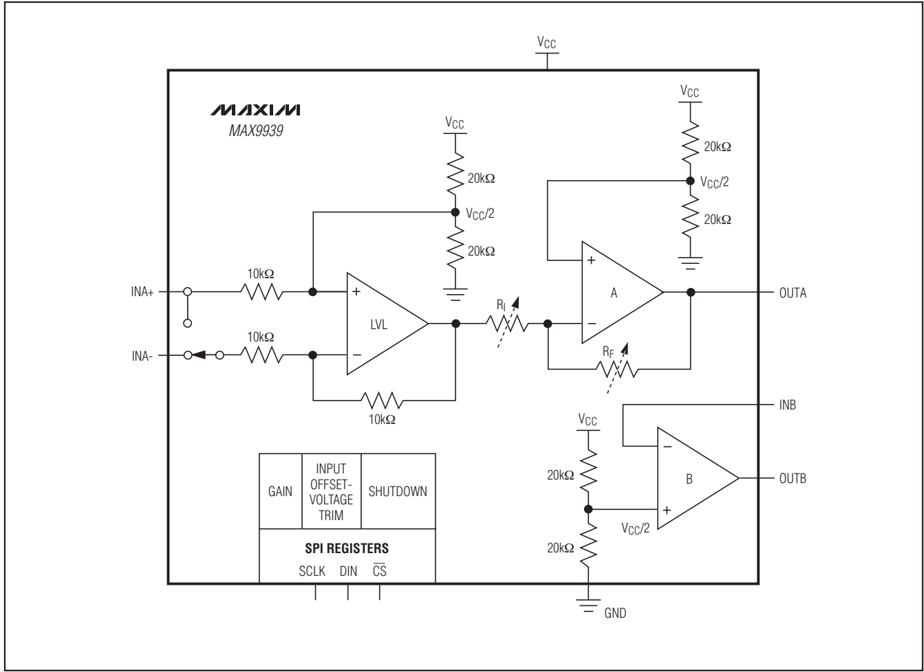
Functional Diagram
