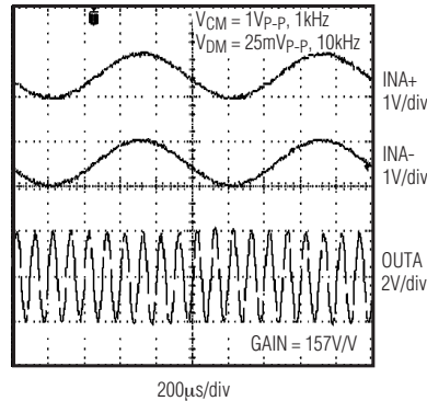
COMMON-MODE REJECTION RESPONSE MAX9939 tac19
