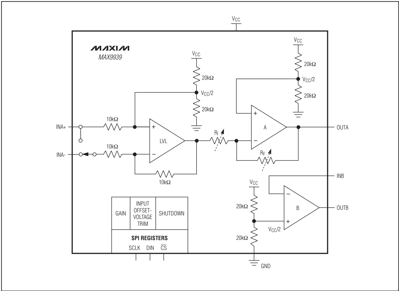
Functional Diagram
