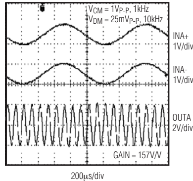
COMMON-MODE REJECTION RESPONSE MAX9939 toc19
