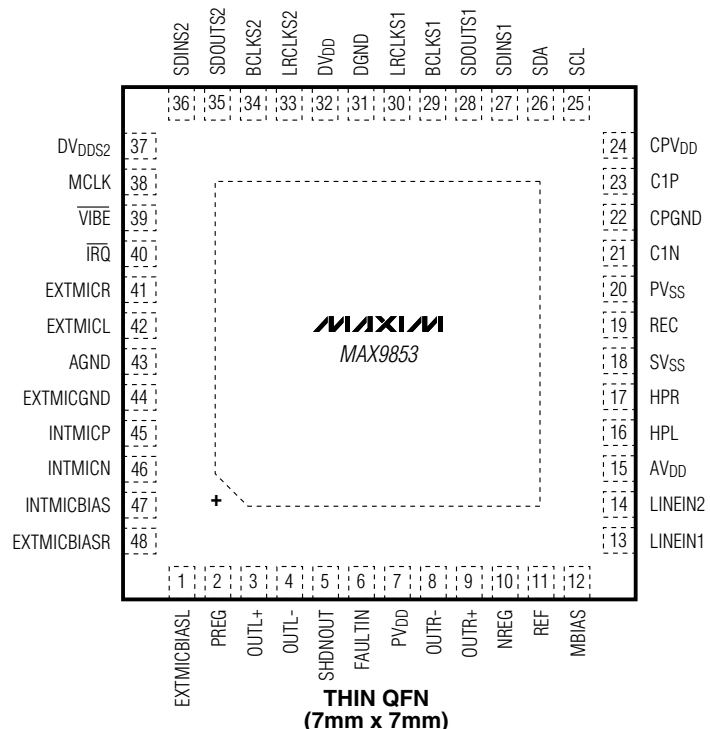
THIN QFN (7mm x 7mm)
