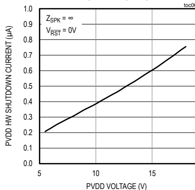
PVDD HARDWARE SHUTDOWN CURRENT vs. PVDD VOLTAGE
