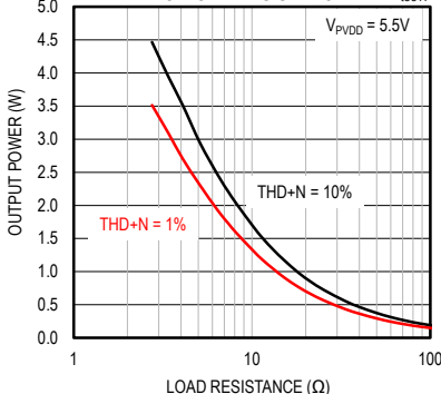
OUTPUT POWER vs. LOAD RESISTANCE
