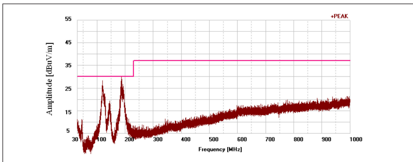
Figure 24. EMI Plot 1: 12in, 8Ω, 16V, 1/2 Power, No Ferrite Bead, Edge Rate +15%
