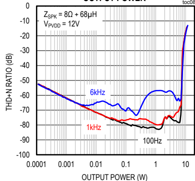
THD+N RATIO vs. OUTPUT POWER
