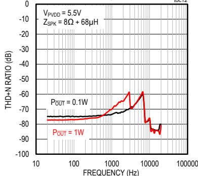
TOTAL HARMONIC DISTORTION PLUS NOISE vs. FREQUENCY
