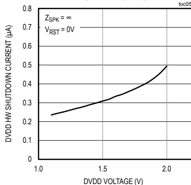
DVDD HARDWARE SHUTDOWN CURRENT vs. DVDD VOLTAGE
