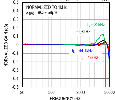
NORMALIZED GAIN vs. FREQUENCY
