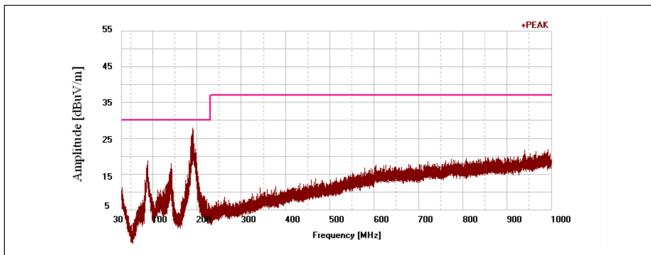
Figure 25. EMI Plot 2: 12in, 4Ω, 16V, 1/2 Power, No Ferrite Bead, Edge Rate +15%
