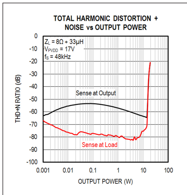
Figure 29. THD Performance Improvement Enabled by Remote Sensing
