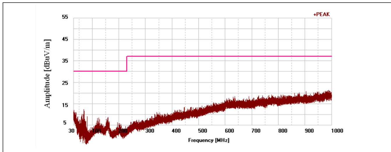
Figure 26. EMI Plot 3: 12in, 8Ω, 16V, ½ Power, Ferrite Bead
