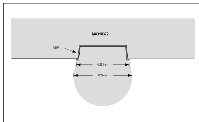
Figure 36. MAX98372+ WLP Ball Dimensions
