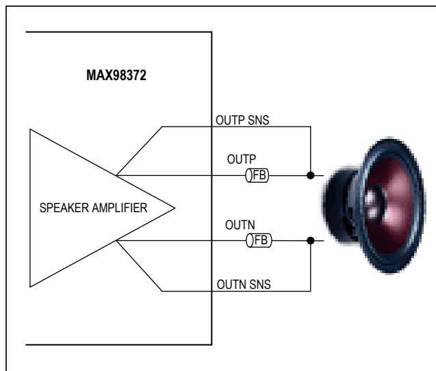
Figure 28. Typical Application Circuit with Ferrites Beads Used
