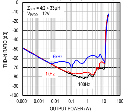
THD+N RATIO vs. OUTPUT POWER
