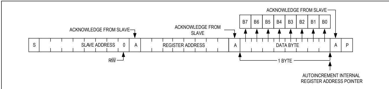
Figure 32. Writing One Byte of Data to the MAX98372
