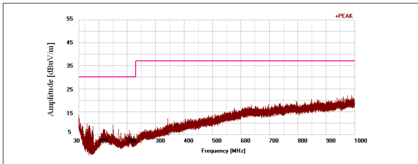
Figure 27. EMI Plot 4: 12in, 4Ω, 16V, ½ Power, Ferrite Bead
