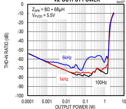
THD+N RATIO vs. OUTPUT POWER
