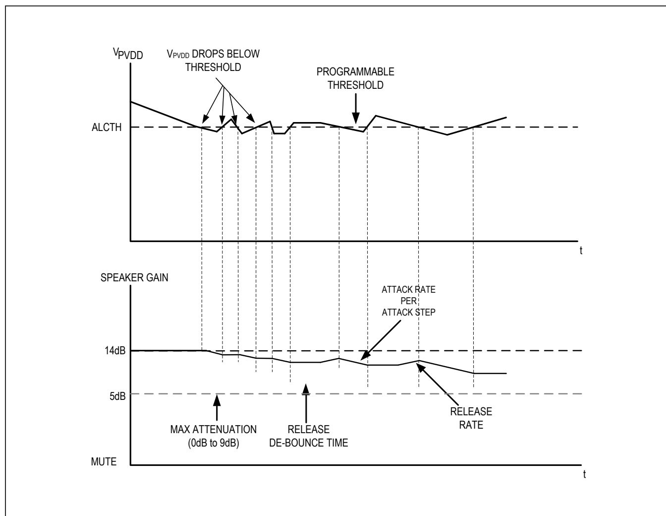
Figure 20. ALC Example 5: Immediate Attenuation
