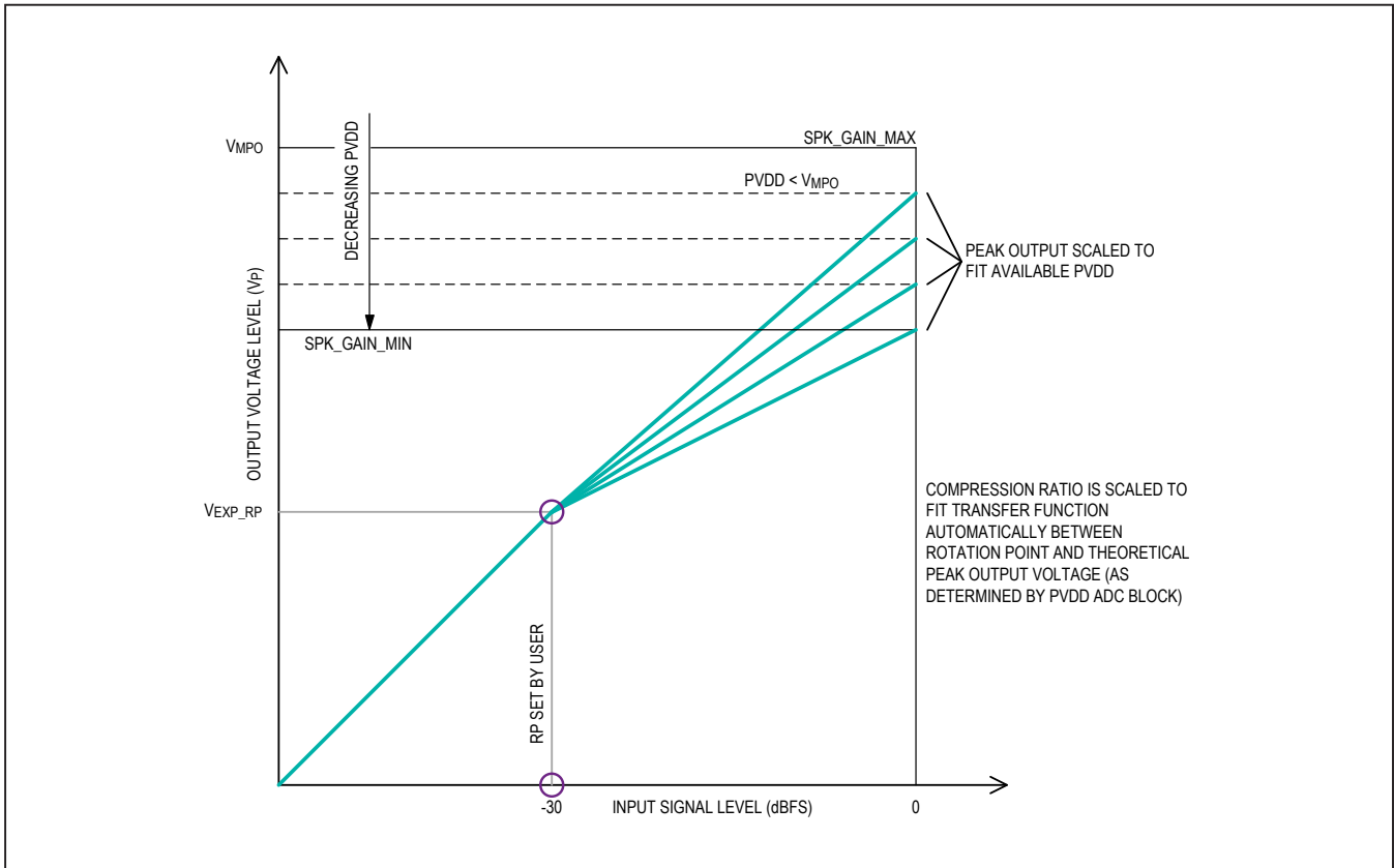
Figure 10. Example of Dynamic Headroom Tracking in Mode 2 Operation with a Low RP
