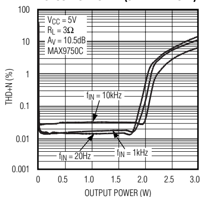
TOTAL HARMONIC DISTORTION PLUS NOISE vs. OUTPUT POWER (SPEAKER MODE)
