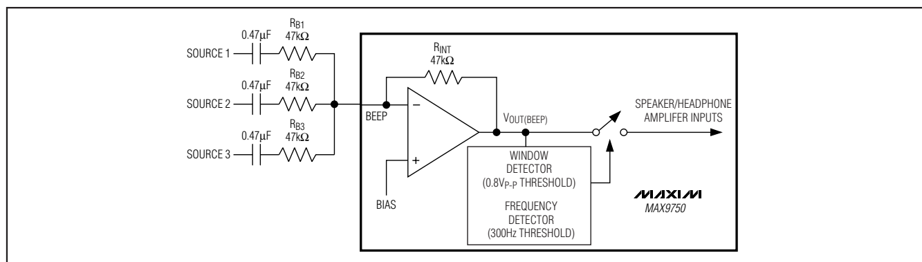
Figure 8. BEEP Input
