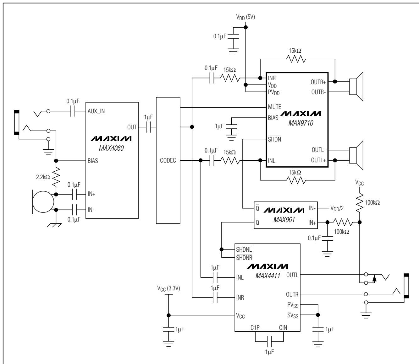
System Diagram
