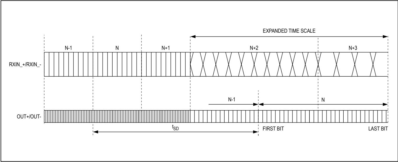
Figure 10. Serializer Delay
