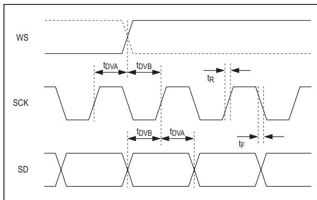
Figure 15. Output I²S Timing Parameters
