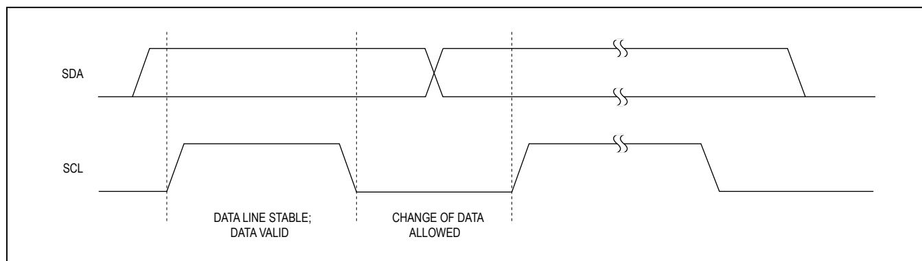
Figure 28. Bit Transfer
