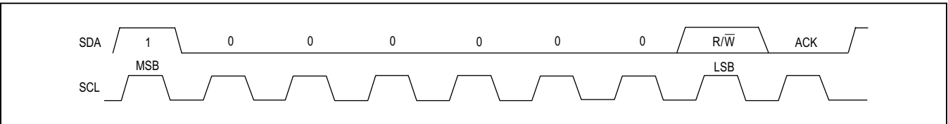
Figure 32. Slave Address
