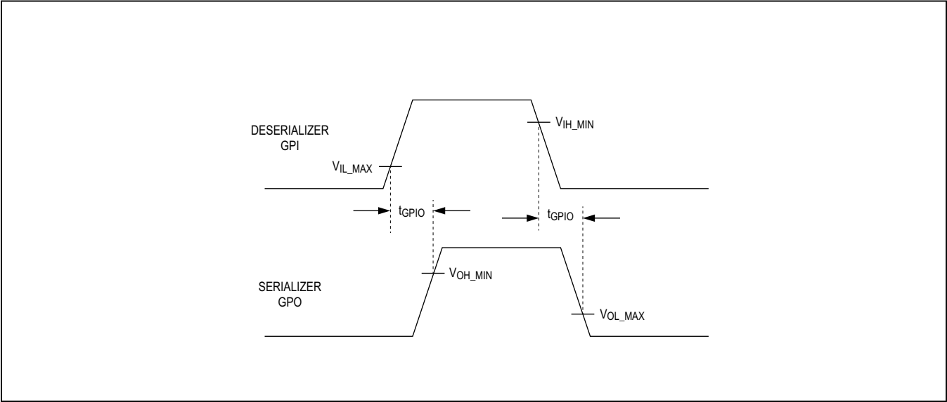
Figure 10. GPI-to-GPO Delay
