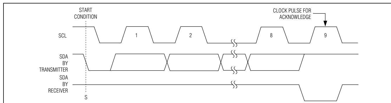
Figure 24. Acknowledge
