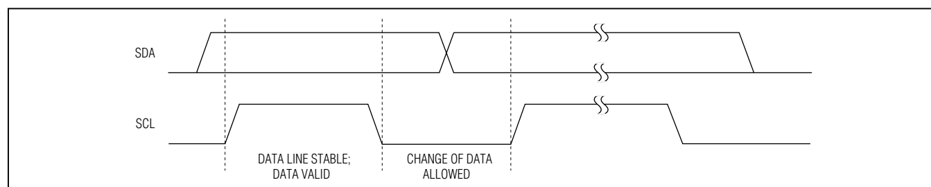
Figure 23. Bit Transfer
