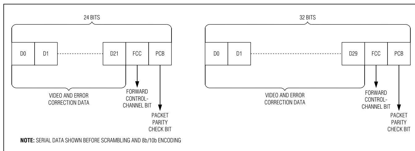
Figure 15. Serial-Data Format
