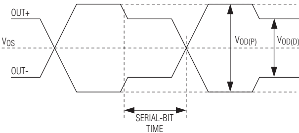
Figure 2. Output Waveforms at OUT+, OUT-
