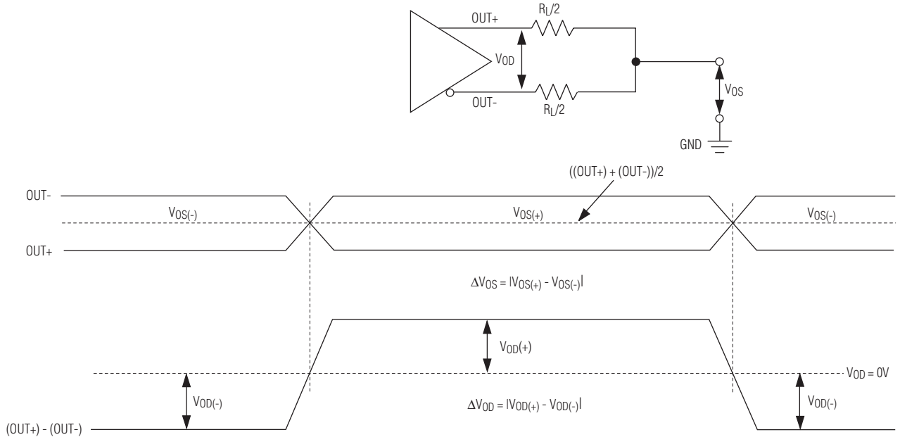
Figure 1. Serial-Output Parameters
