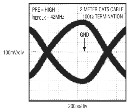
EYE DIAGRAM WITH PREEMPHASIS
