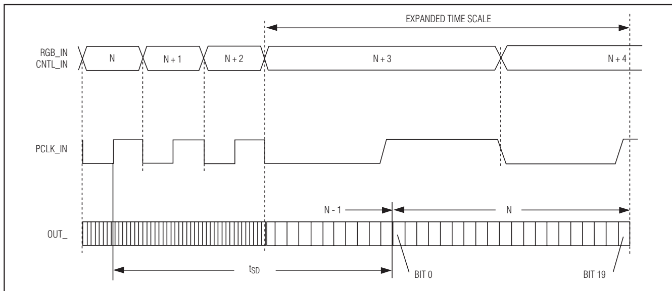
Figure 5. Serializer Delay
