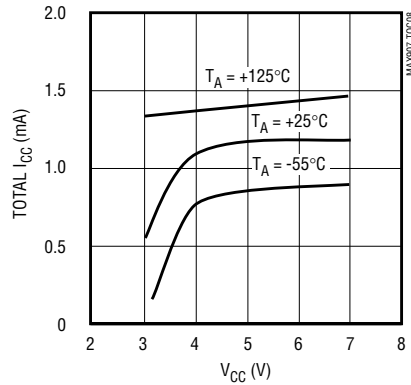
MAX907 TOTAL POSITIVE SUPPLY CURRENT vs. POSITIVE SUPPLY VOLTAGE (OUTPUTS AT V_OH)
