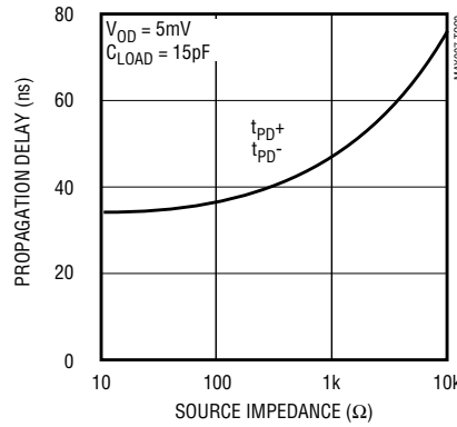
PROPAGATION DELAY vs. SOURCE IMPEDANCE
