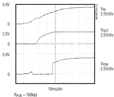
POK STARTUP RESPONSE
