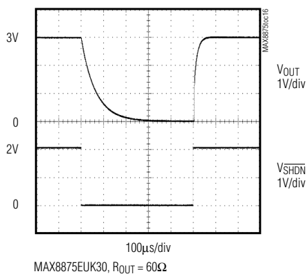
SHUTDOWN DELAY
