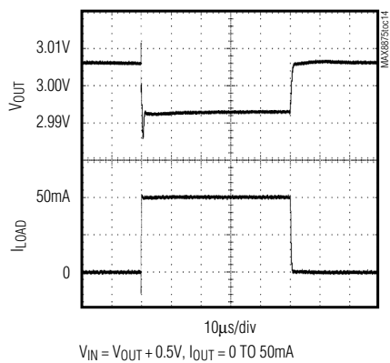
LOAD-TRANSIENT RESPONSE
