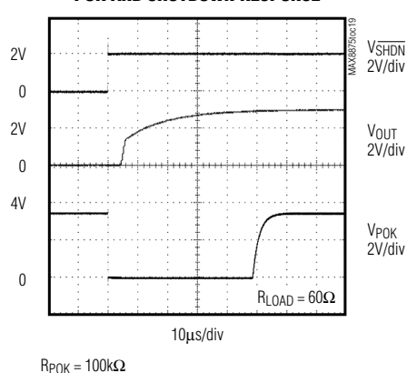
POK AND SHUTDOWN RESPONSE
