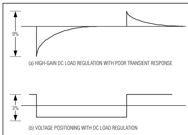
Figure 3. Transient-Response Comparison
