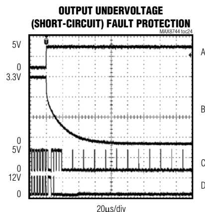
A. LOAD FET GATE, 5V/div B. 3.3V OUTPUT ( V_{OUT3} ), 1V/div 30m \Omega MOSFET C. DL3, 5V/div D. DH3, 10V/div
