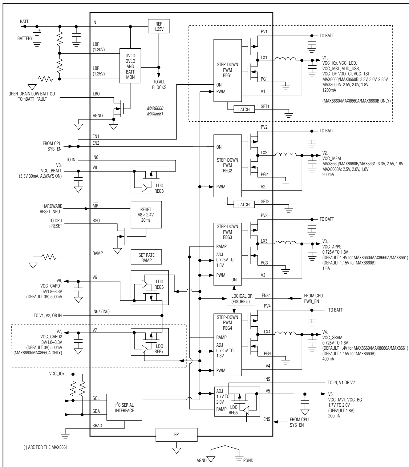
Figure 2. Functional Diagram
