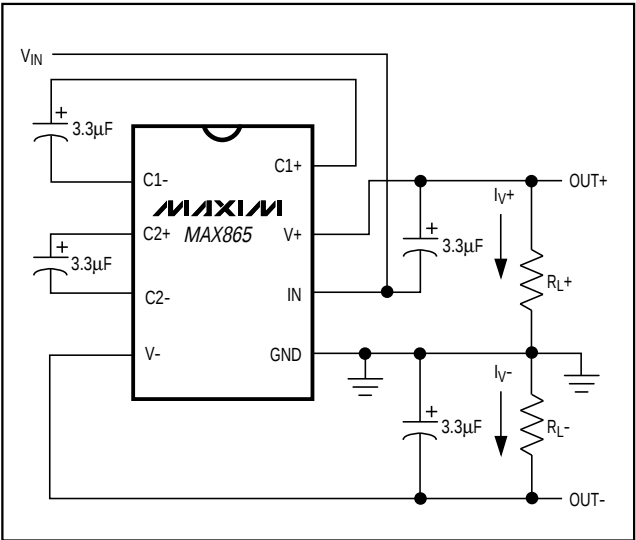
Figure 1. Test Circuit
