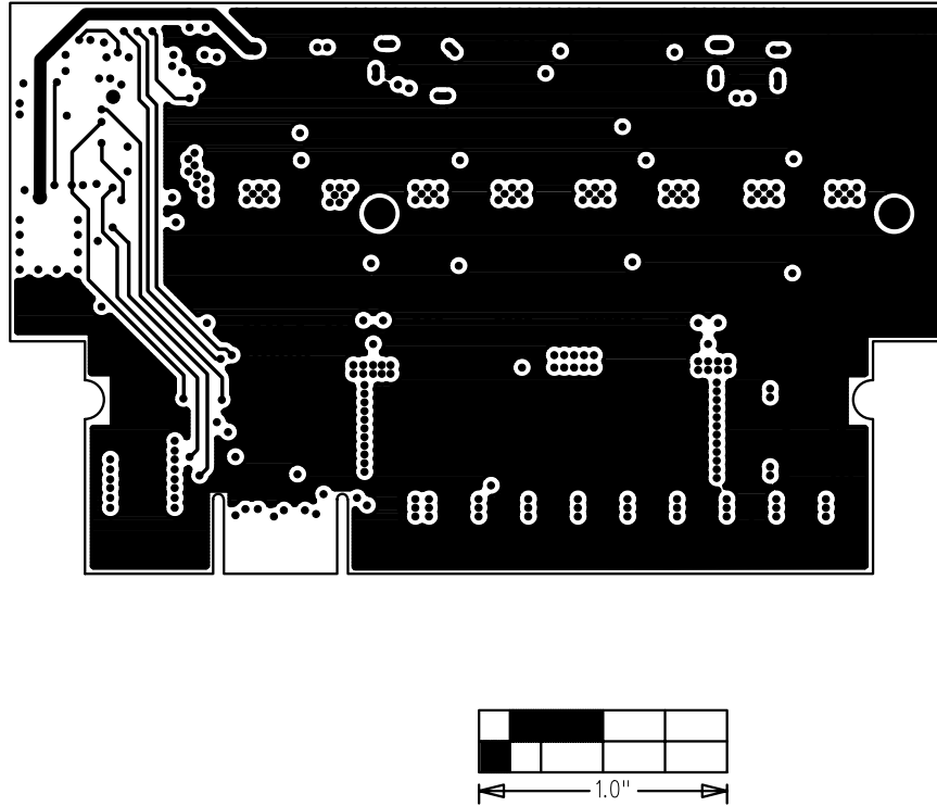
Figure 8. MAX8525 EV Kit PC Board Layout—GND Layer 5
