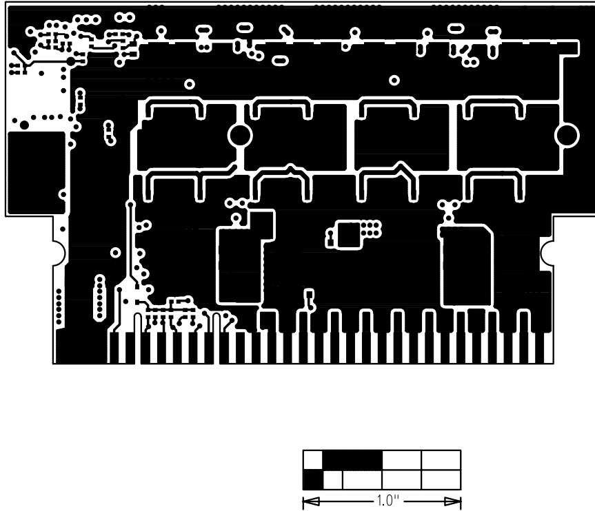
Figure 9. MAX8525 EV Kit PC Board Layout—Solder Side
