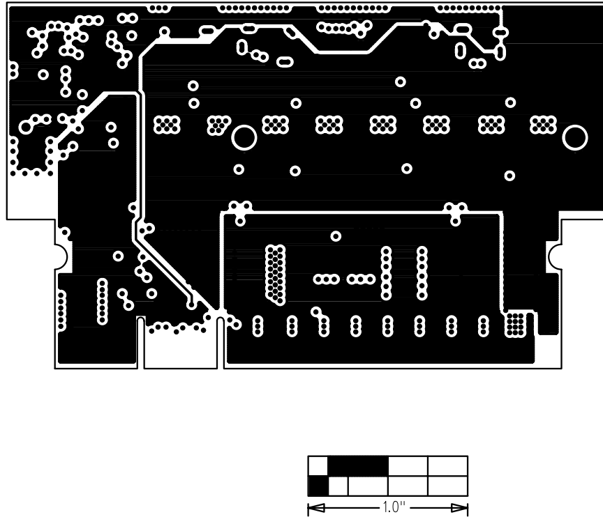
Figure 6. MAX8525 EV Kit PC Board Layout—GND Layer 3
