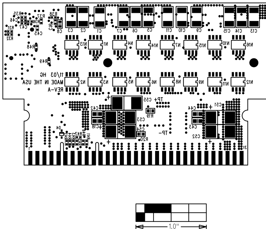
Figure 10. MAX8525 EV Kit Component Placement Guide—Solder Side
