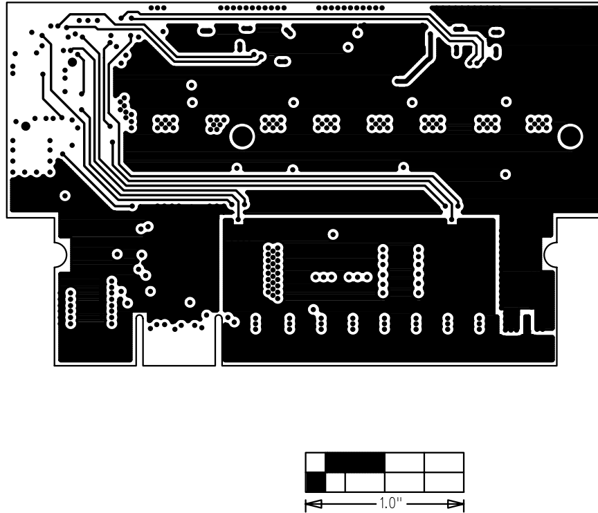
Figure 7. MAX8525 EV Kit PC Board Layout—SENSE/GND Layer 4
