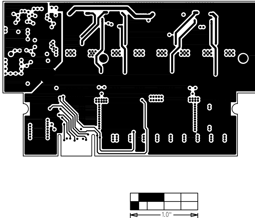
Figure 5. MAX8525 EV Kit PC Board Layout—GND Layer 2
