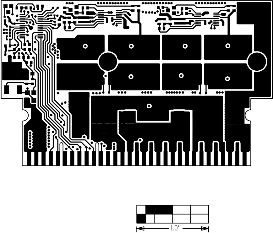
Figure 4. MAX8525 EV Kit PC Board Layout—Component Side
