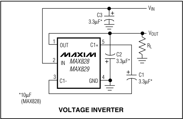
Figure 1. Test Circuit
