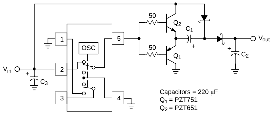
Figure 48. Positive Output Voltage Doubler with High Current Capability
