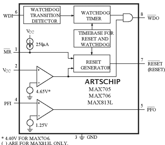
Figure 1. MAX705/MAX706/MAX813L Block Diagram
