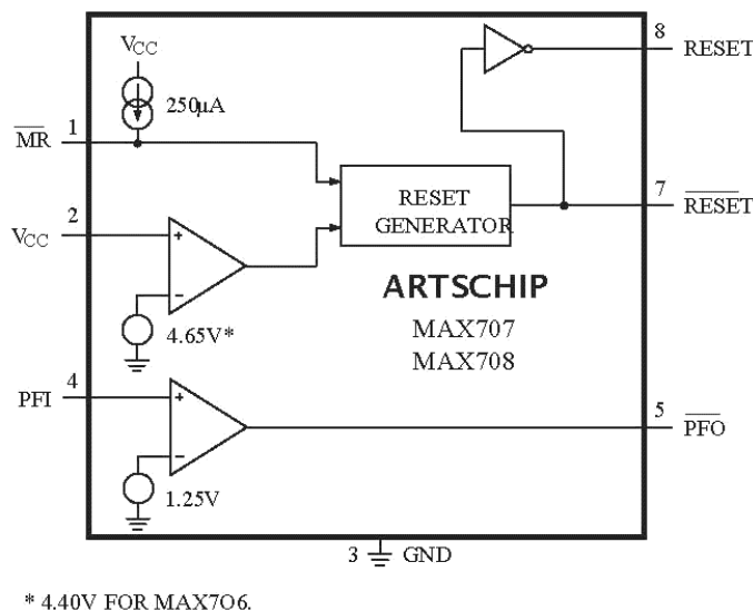
Figure 2. MAX707/MAX708 Block Diagram
