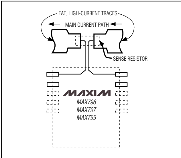
Figure 10. Kelvin Connections for the Current-Sense Resistor
