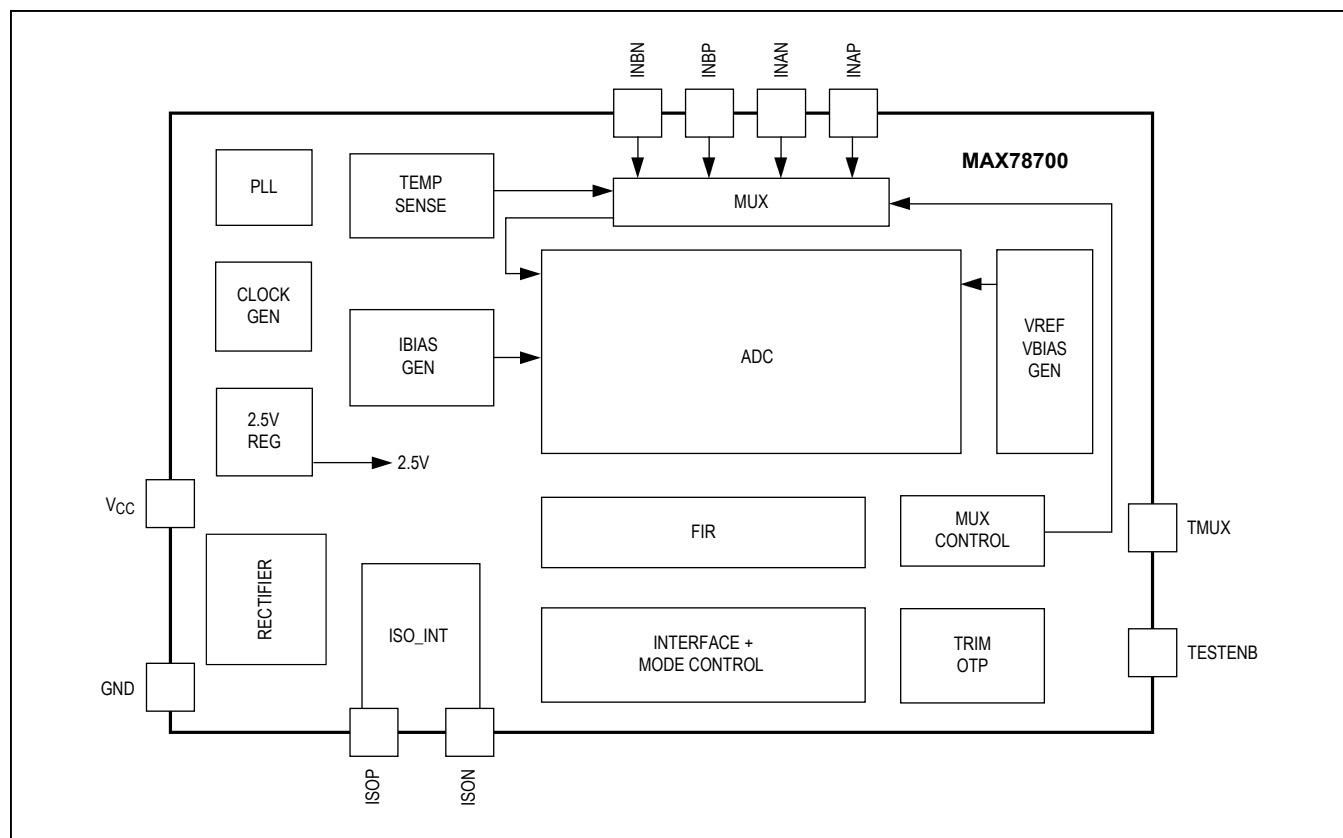
Figure 1. Functional Diagram
